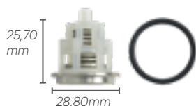
Kit Dolly 169, valves + O-ring
