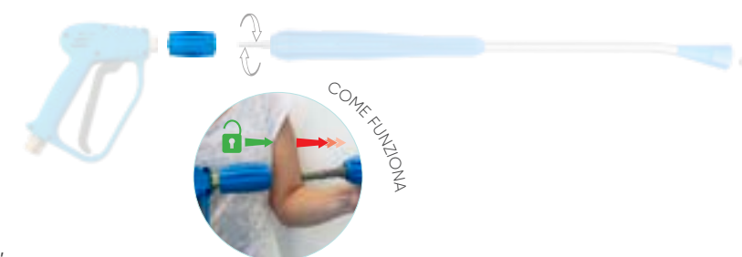
F swivel ball quick coupling AISI 304 stainless steel KW type, inlet G1/4" M
