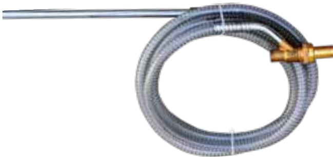
Professional sandblasting kit, inlet G1/4" F, 250bar, 40l/min. Complete with brass sandblasting head with WIDIA insert, 4m suction hose and galvanised steel probe
