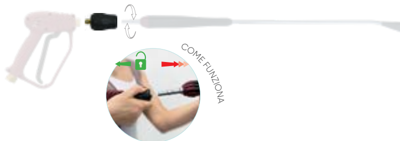
REVERSE F swivel ball quick coupling KW type, inlet G1/4" M
